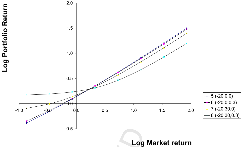
Fig. 4. Expected NMW = -20.
