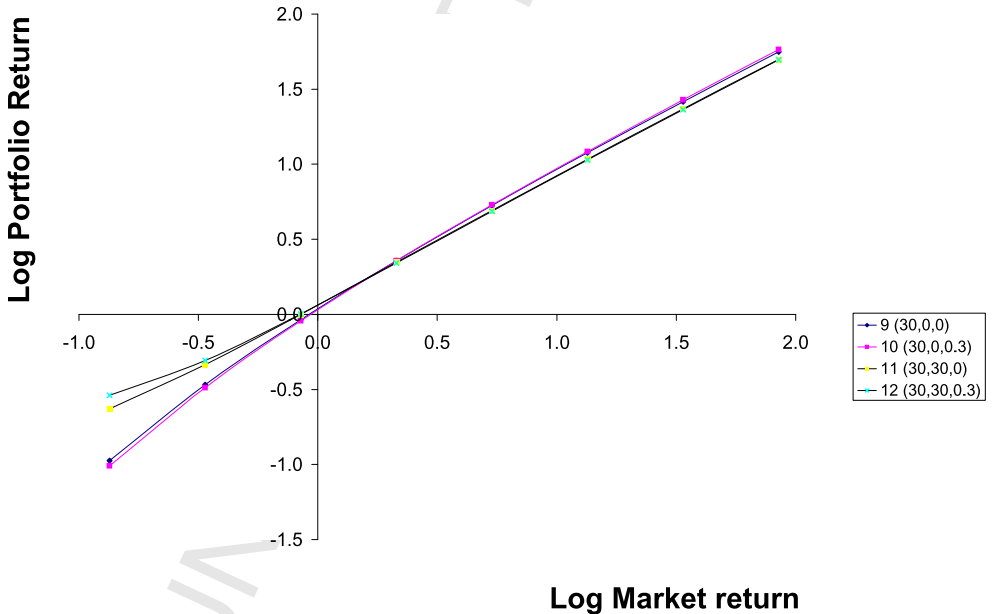
Fig. 5. Expected NMW = 30.
