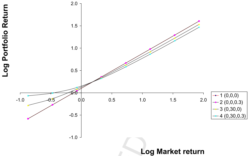
Fig. 3. Expected NMW = 0.
