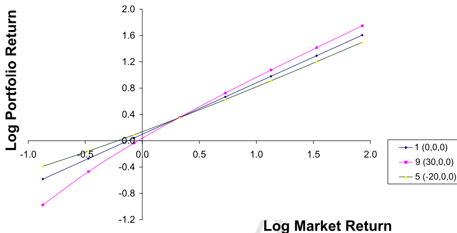
Fig. 2. Non-stochastic NMW.
